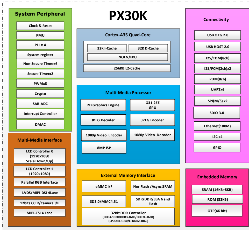
Fig.1-2 Block Diagram
